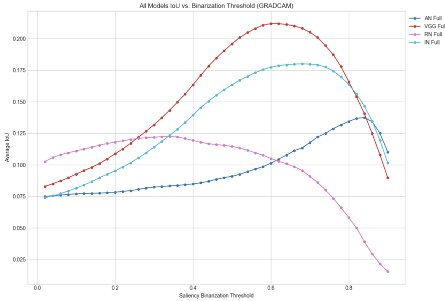
Figure 7: Model-Expert IoUs vs. Thresholds (Grad-CAM). IoU between model saliency maps and expert annotations as a function of the binarization threshold applied to Grad-CAM outputs.
