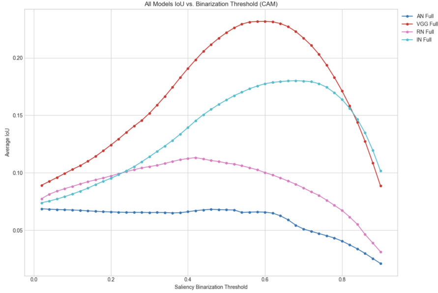
Figure 6: Model-Expert IoUs vs. Thresholds (CAM). IoU between model saliency maps and expert annotations as a function of the binarization threshold applied to CAM outputs.
